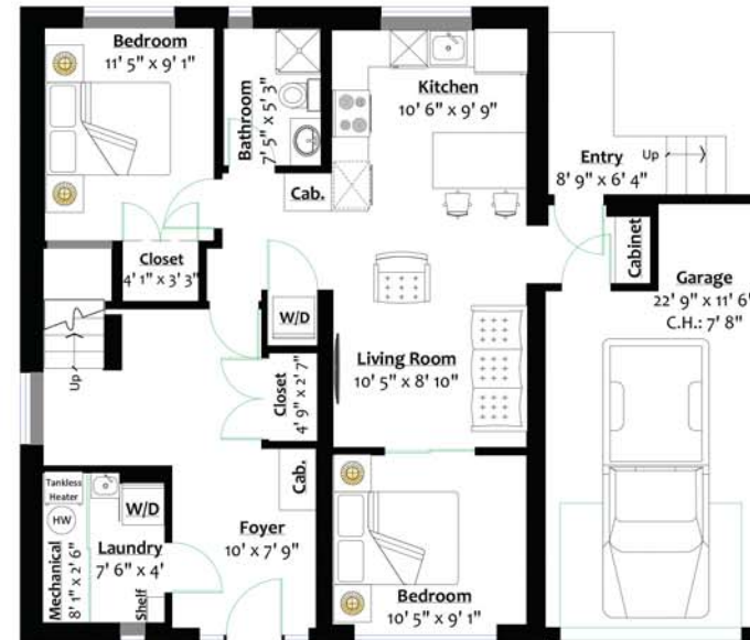
LOWER LEVEL Floor Area: 999 Sq. Ft. Ceiling Height: 7' 9"
